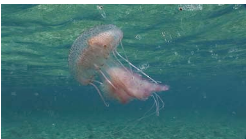
medusa ( Pelagia noctiluca )
